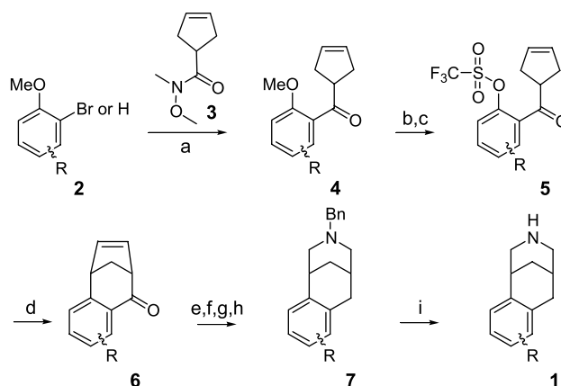
Scheme 1. Reagents and conditions: (a) [1] n -BuLi, THF -78 to 20 °C [2] HCl ( >90\% ); (b) BCl_3 , CH_2Cl_2 ; (c) (CF_3SO_2)_2O , pyr, CH_2Cl_2 (55–85%); (d) 4 mol % Pd(OAc)_2 , 10 mol % Ph_3P(CH_2)_3PPh_3 , 20 mol % KOAc, 1.5 equiv Et_3N , DMF, 1–3 h, 110 °C (57–85%); (e) NH_2NH_2 , KOH, (HOCH_2)_2 , \Delta (93%); (f) OsO_4 , (CH_2)_5NCH_3O \cdot H_2O acetone, H_2O ; (g) NaIO_4 , ClCH_2CH_2Cl/H_2O ; (h) BnNH_2 , ClCH_2CH_2Cl , NaBH(OAc)_3 (30–78%); (i) NH_4HCO_2 , Pd(OH)_2 , MeOH, \Delta (30–90%).
