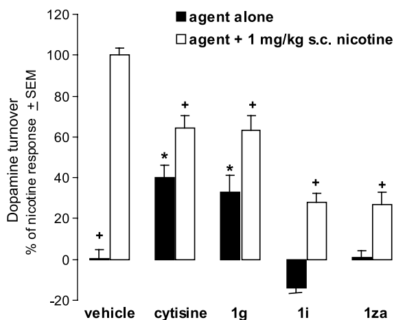
Figure 1. Effects of nicotine, (–)-cytisine, 1g , 1i , and 1za on dopamine turnover in rat nucleus accumbens 1 h post-dose. All values are normalized to the effect of 1.0 mg/kg s.c. nicotine (=100%). Compounds were administered alone (at maximum tolerated doses [filled bars]) of (–)-cytisine, 5.6 mg/kg; 1g , 8 mg/kg; 1i , 10 mg/kg; and 1za , 5 mg/kg and concurrently with 1 mg/kg s.c. nicotine (open bars). Mean nicotine increase alone = 177% control; N = 5–10 (all agents alone: *p < .05 compared to vehicle; all agents with nicotine: +p < .05 compared to nicotine, One-Way ANOVA, post hoc, Dunnett's). Doses were selected through experimental determination of behavioral limited ceilings for each agent alone and in combination.
